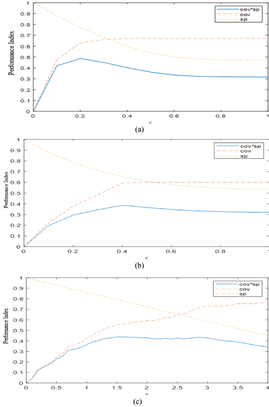
Fig. 4. Values of performance index V obtained for successive values of \epsilon . Using (a) protocol 1, (b) protocol 2, and (c) protocol 3.
