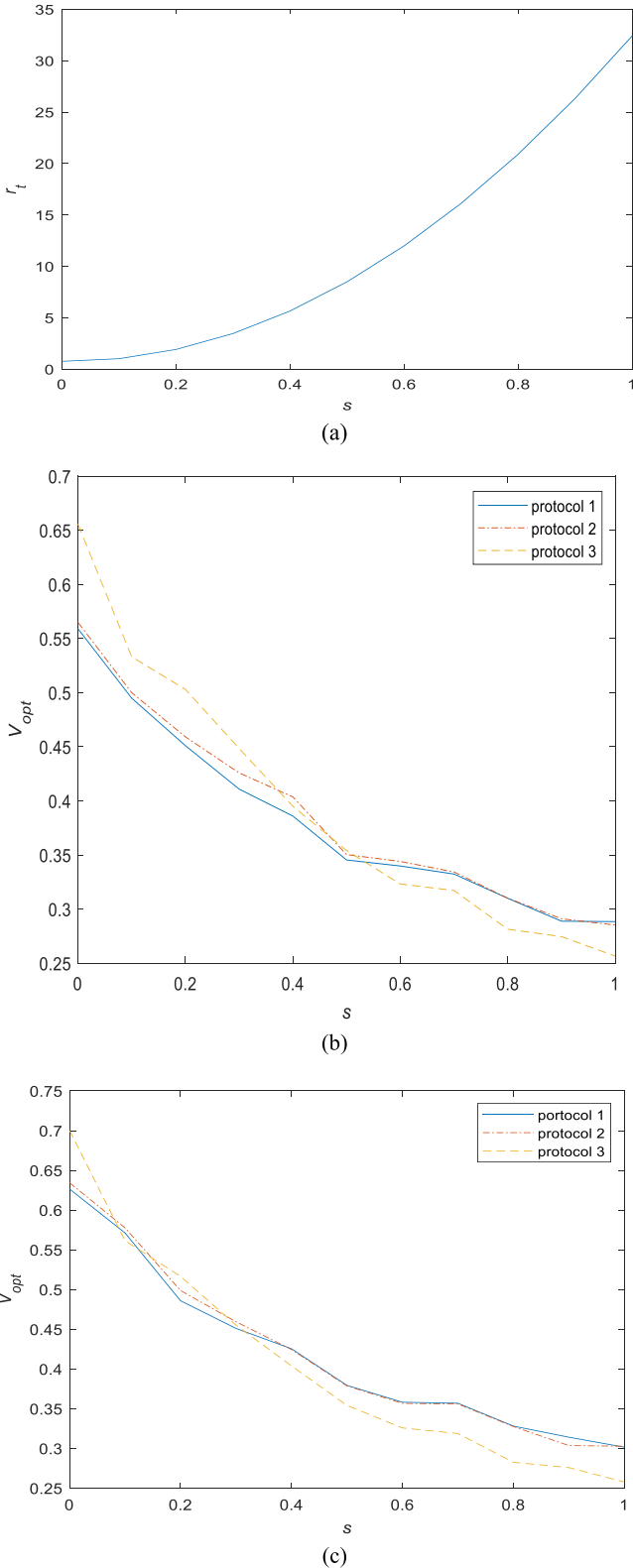
Fig. 7. Performance index as a function of \sigma for (a) ratio r_t (b) V_{opt} (uniform \epsilon ) and (c) V_{opt} (non-uniform \epsilon ) s : x-axis represents the variation of \sigma from 0 to 1.
