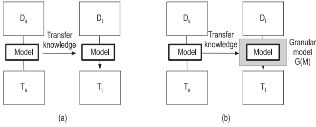
Fig. 1. Transfer learning (a) and granular transfer learning: a paradigm shift (b) Note the emergence of a granular model in the target domain.
