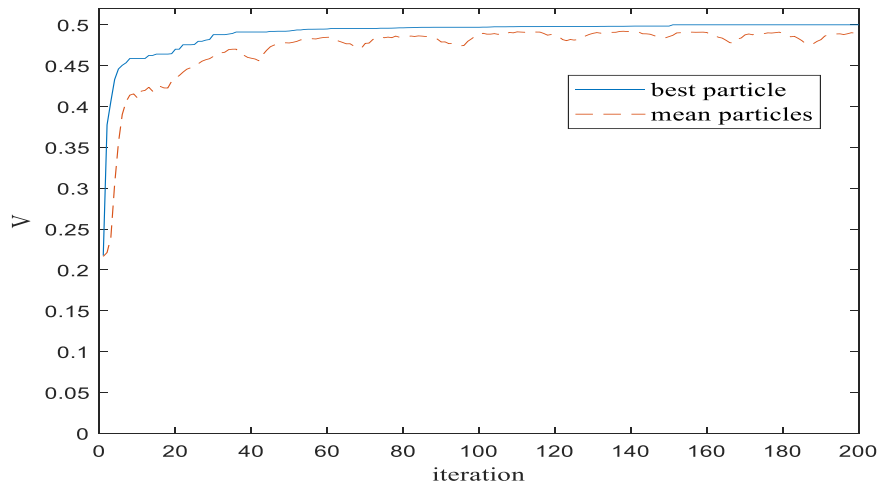
Fig. 6. Convergence of PSO in successive iterations.
