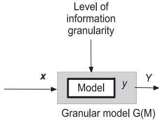
Fig. 2. From numeric to granular model: optimized level of information granularity \varepsilon serves as a design asset.
