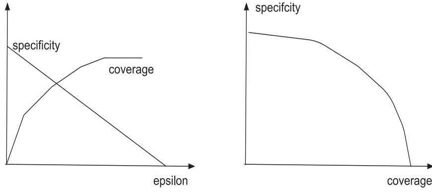
Fig. 3. An example plot of coverage and specificity treated as functions of \epsilon . The optimal value \epsilon is attained when the product \overline{cov} * \overline{sp} attains maximal value.
